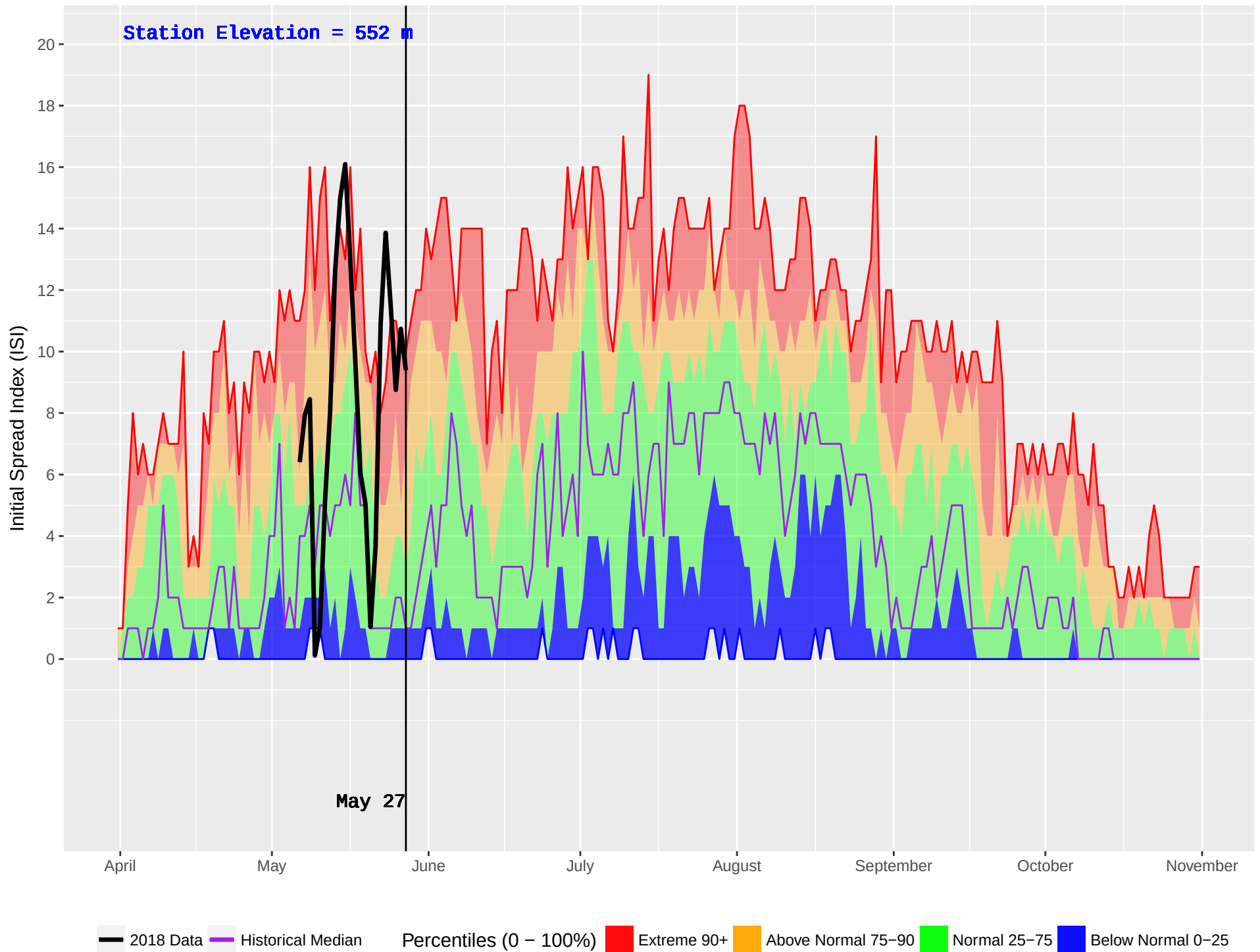
NAHATLATCH (316) : Historical (2001–2016) and Current (2018) Noon Initial Spread Index (ISI)
