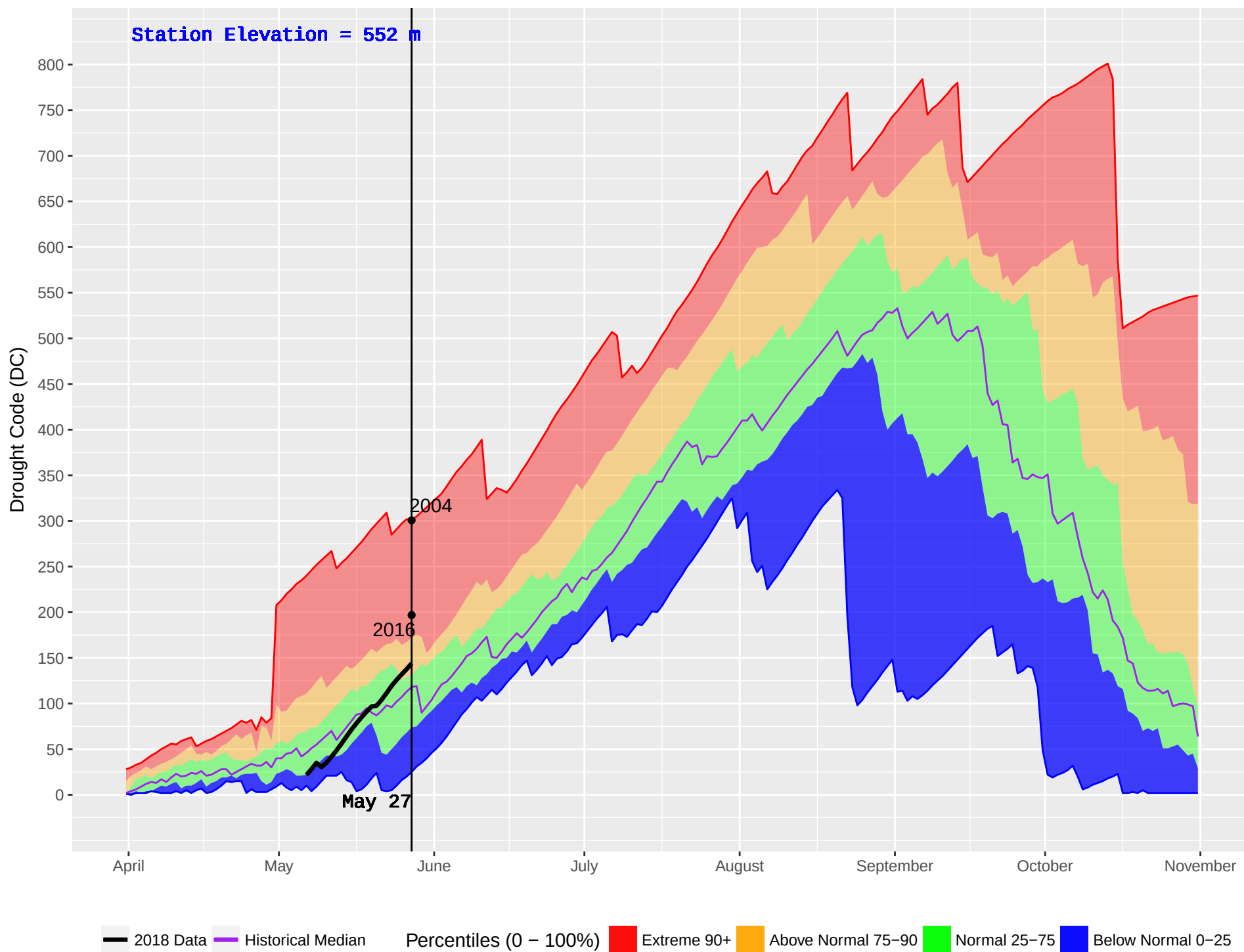
NAHATLATCH (316) : Historical (2001–2016) and Current (2018) Noon Drought Code (DC)
